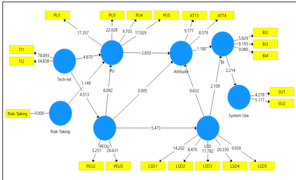
Figure 2. Model Bootstrapping
